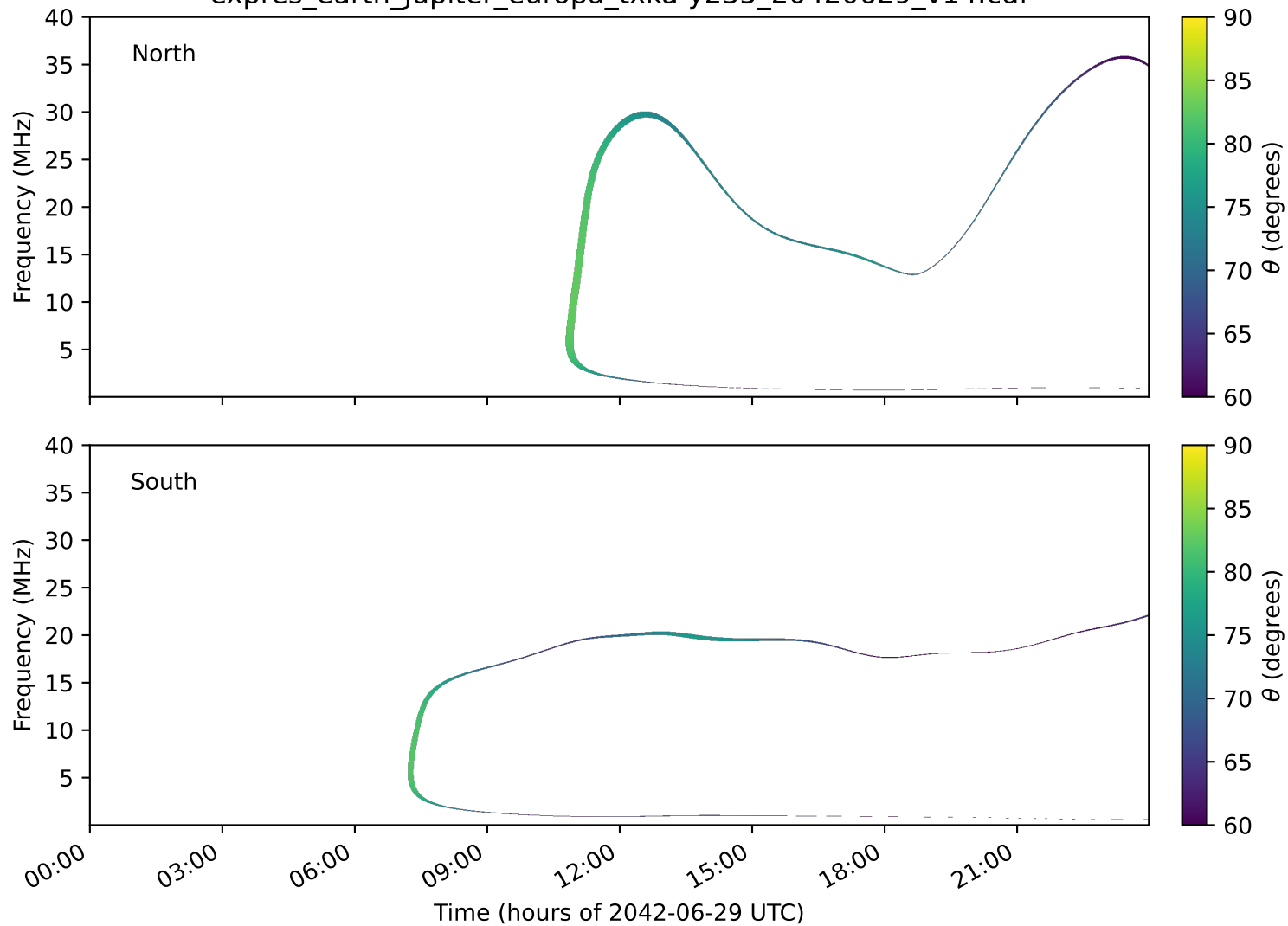
expres_earth_jupiter_europa_txka-y235_20420629_v14.cdf
