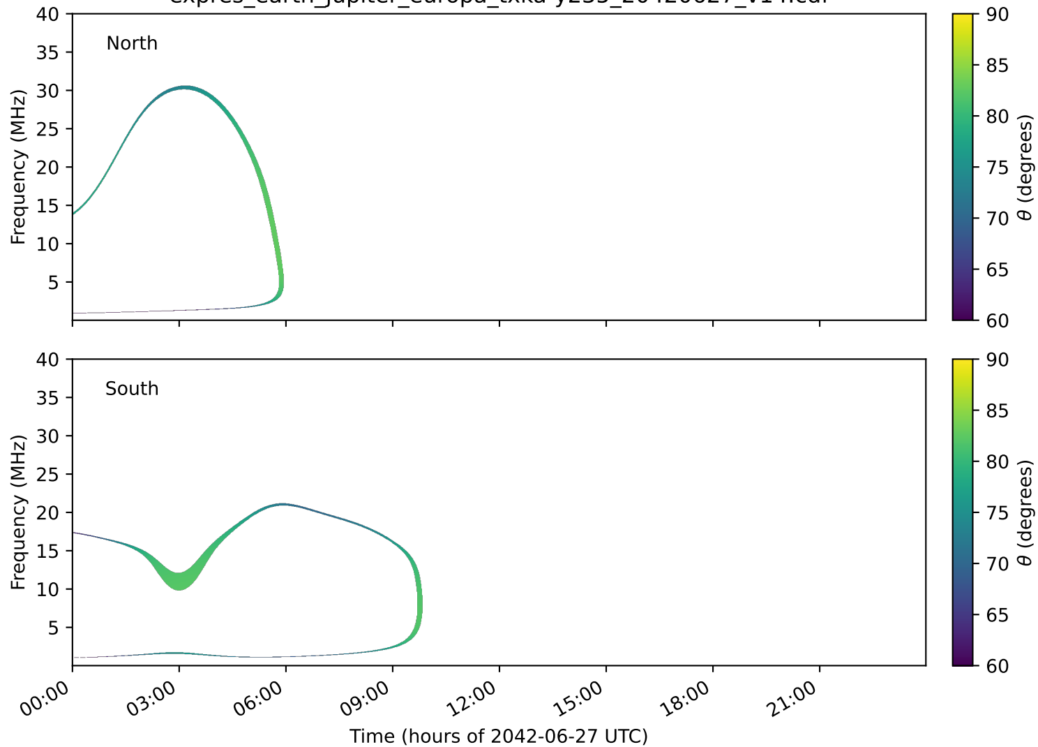
expres_earth_jupiter_europa_txka-y235_20420627_v14.cdf
