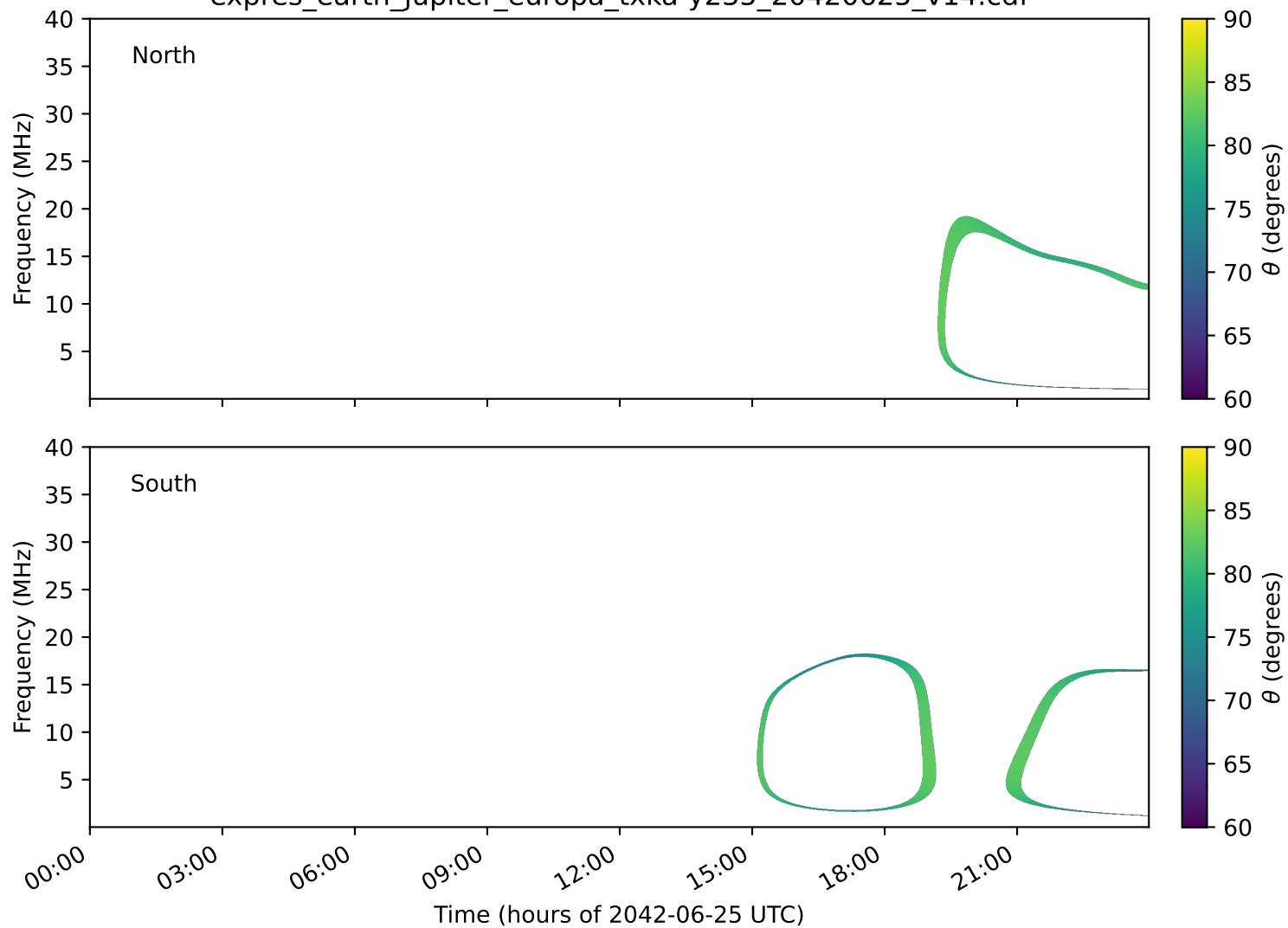
expres_earth_jupiter_europa_txka-y235_20420625_v14.cdf
