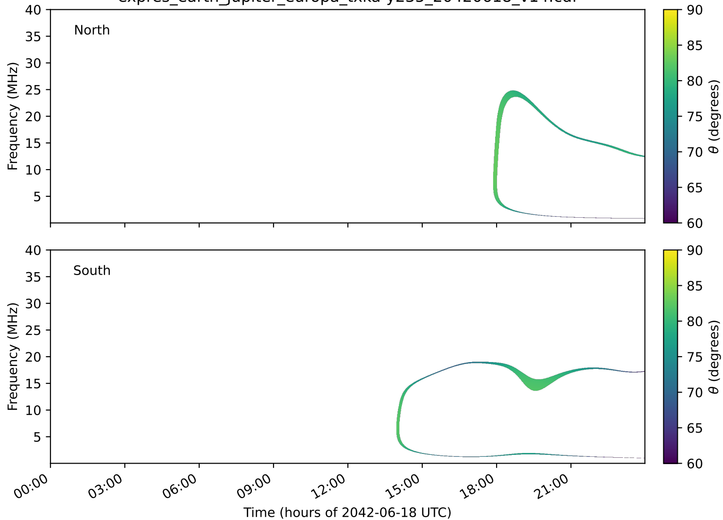
expres_earth_jupiter_europa_txka-y235_20420618_v14.cdf
