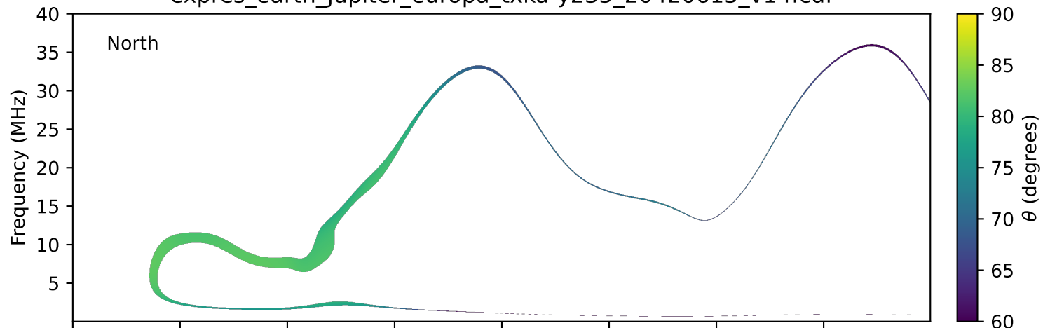
expres_earth_jupiter_europa_txka-y235_20420615_v14.cdf
