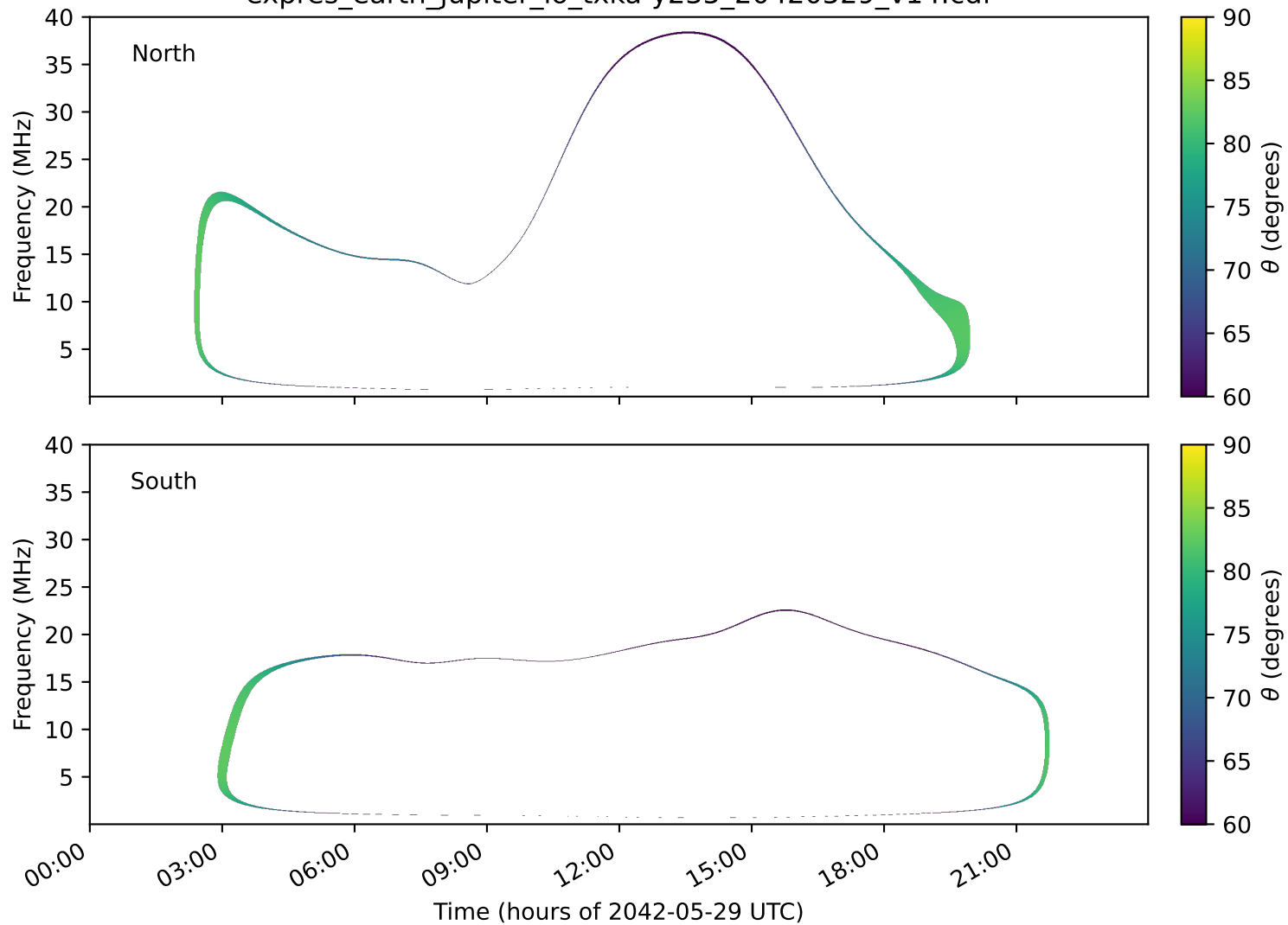
expres_earth_jupiter_io_txka-y235_20420529_v14.cdf
