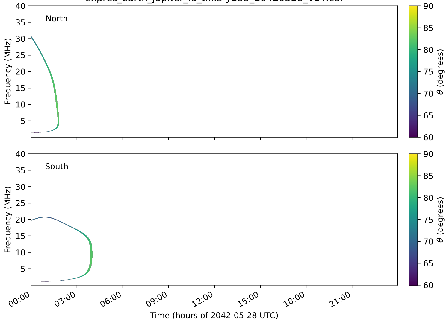
expres_earth_jupiter_io_txka-y235_20420528_v14.cdf
