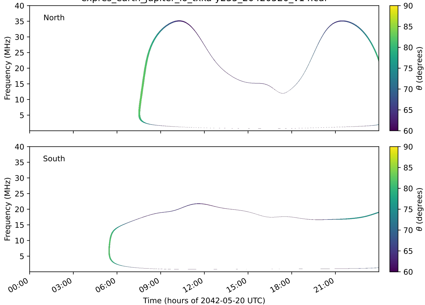
expres_earth_jupiter_io_txka-y235_20420520_v14.cdf
