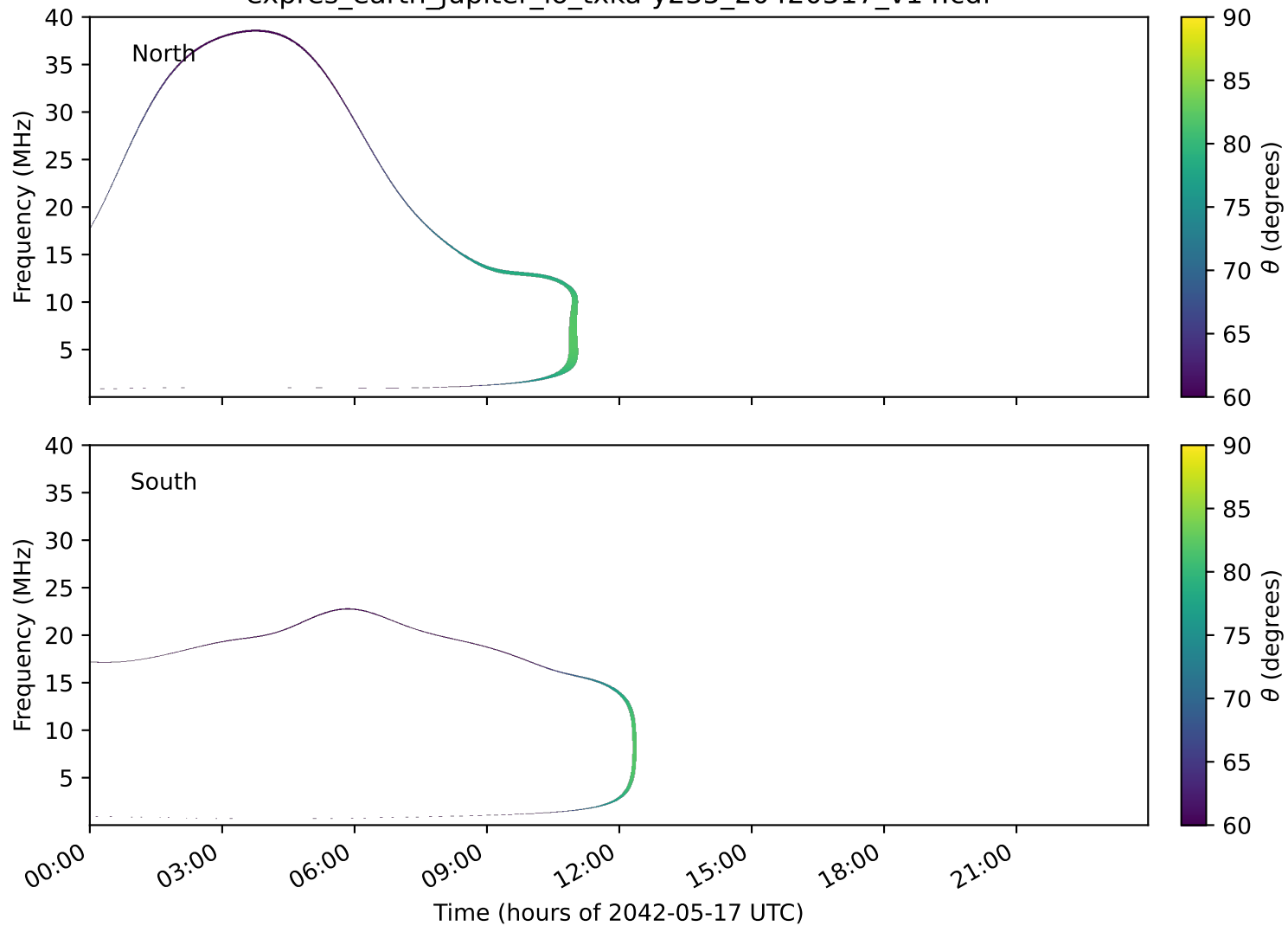
expres_earth_jupiter_io_txka-y235_20420517_v14.cdf
