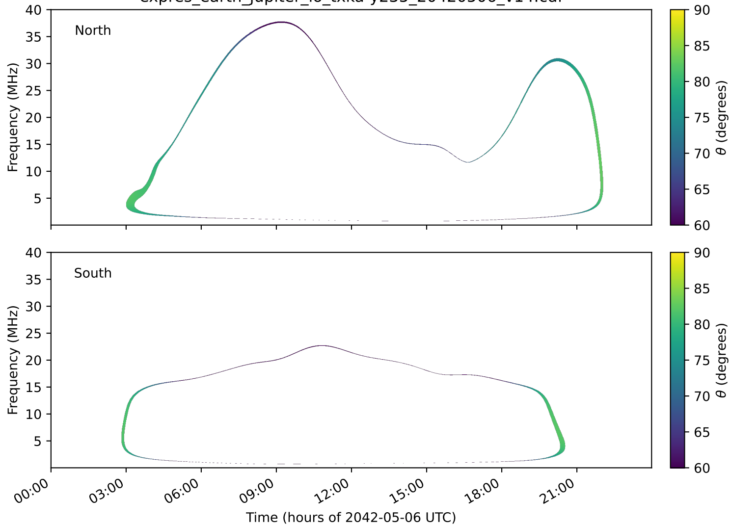
expres_earth_jupiter_io_txka-y235_20420506_v14.cdf
