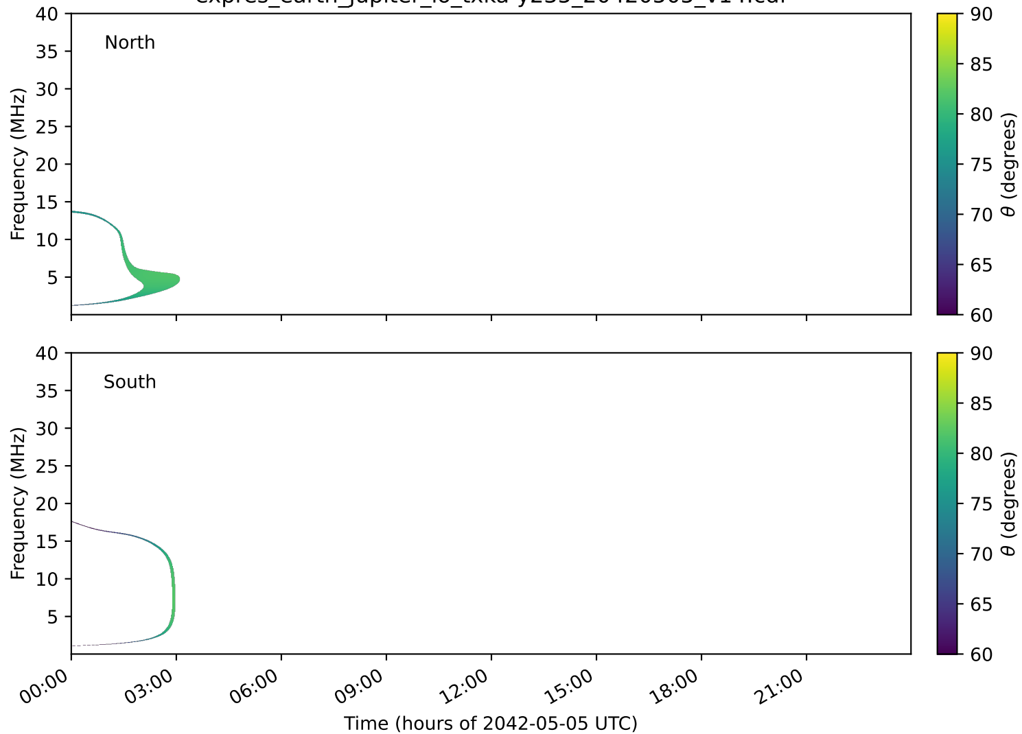
expres_earth_jupiter_io_txka-y235_20420505_v14.cdf
