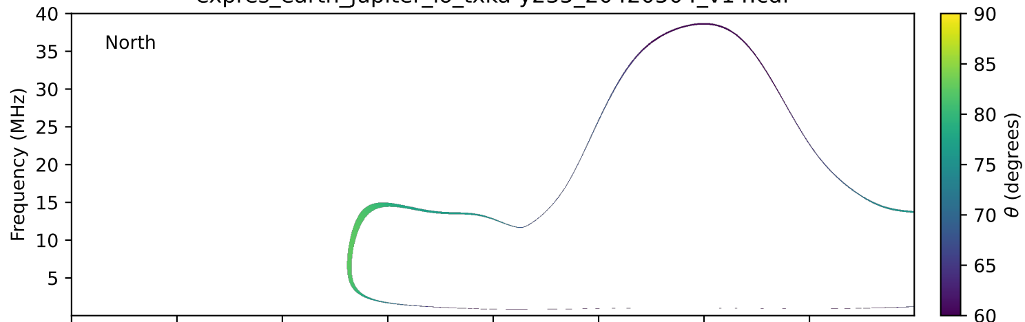
expres_earth_jupiter_io_txka-y235_20420504_v14.cdf
