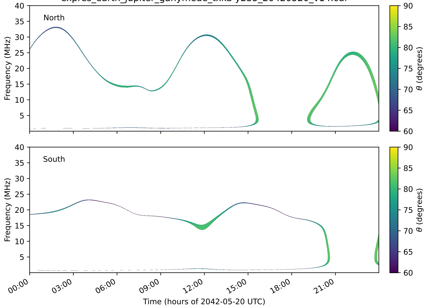
expres_earth_jupiter_ganymede_txka-y235_20420520_v14.cdf
