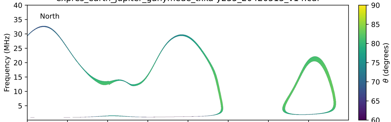
expres_earth_jupiter_ganymede_txka-y235_20420513_v14.cdf
