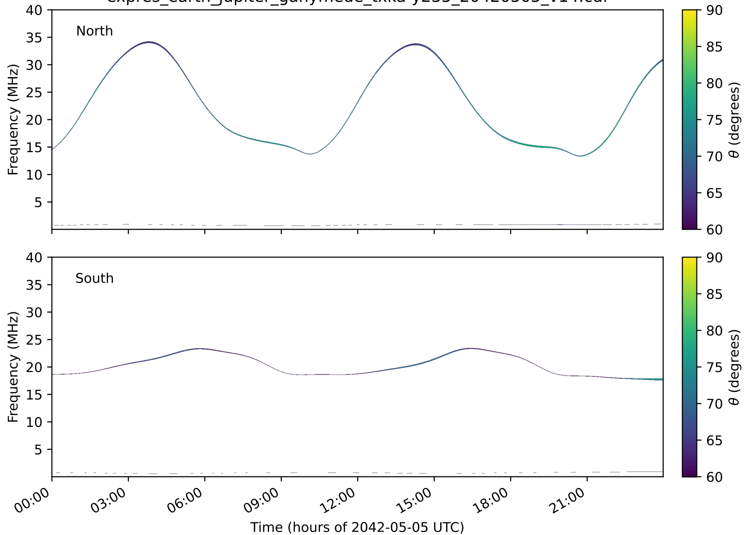
expres_earth_jupiter_ganymede_txka-y235_20420505_v14.cdf
