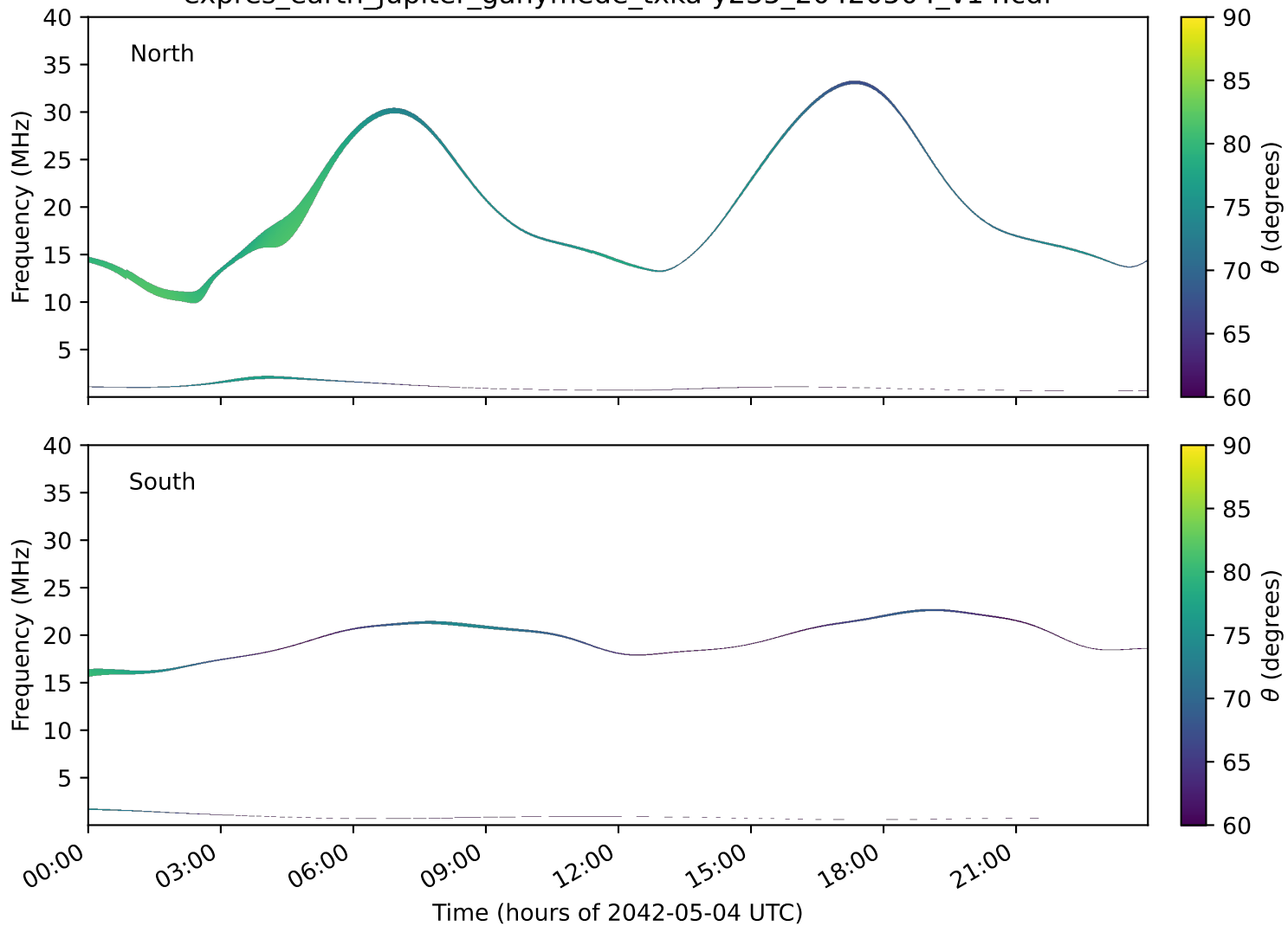
expres_earth_jupiter_ganymede_txka-y235_20420504_v14.cdf
