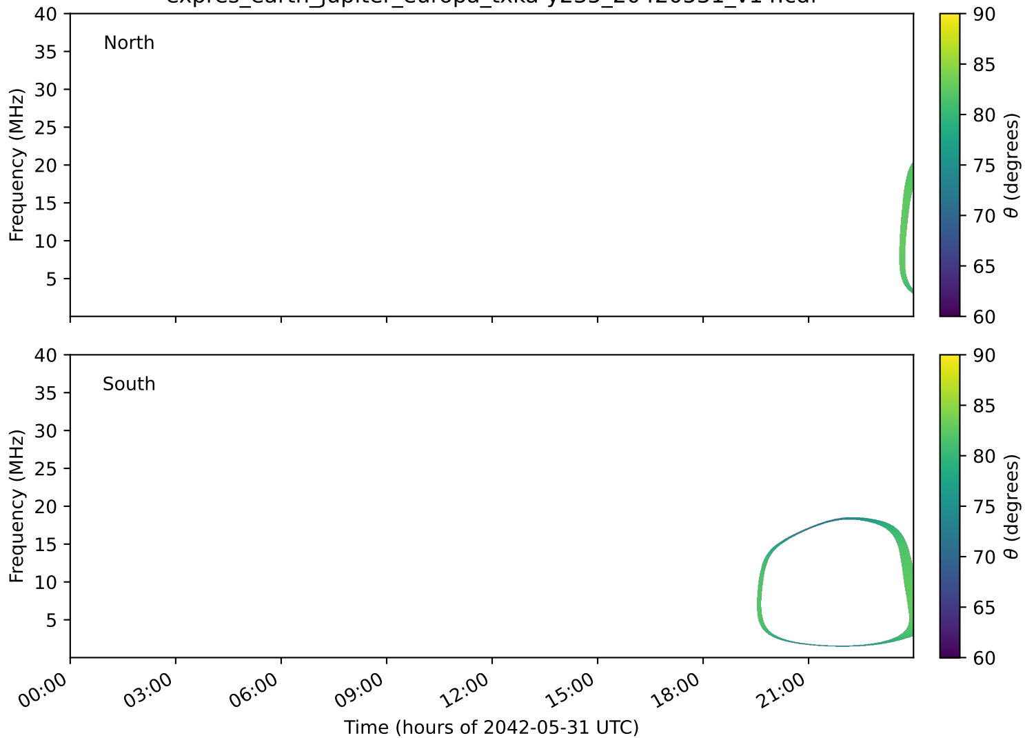
expres_earth_jupiter_europa_txka-y235_20420531_v14.cdf
