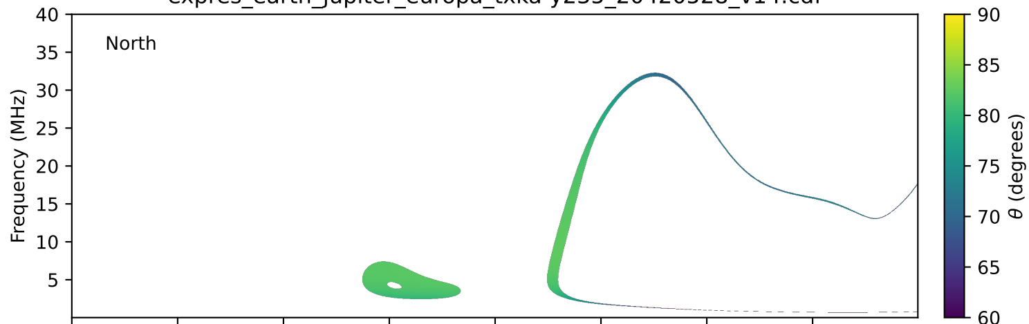
expres_earth_jupiter_europa_txka-y235_20420528_v14.cdf
