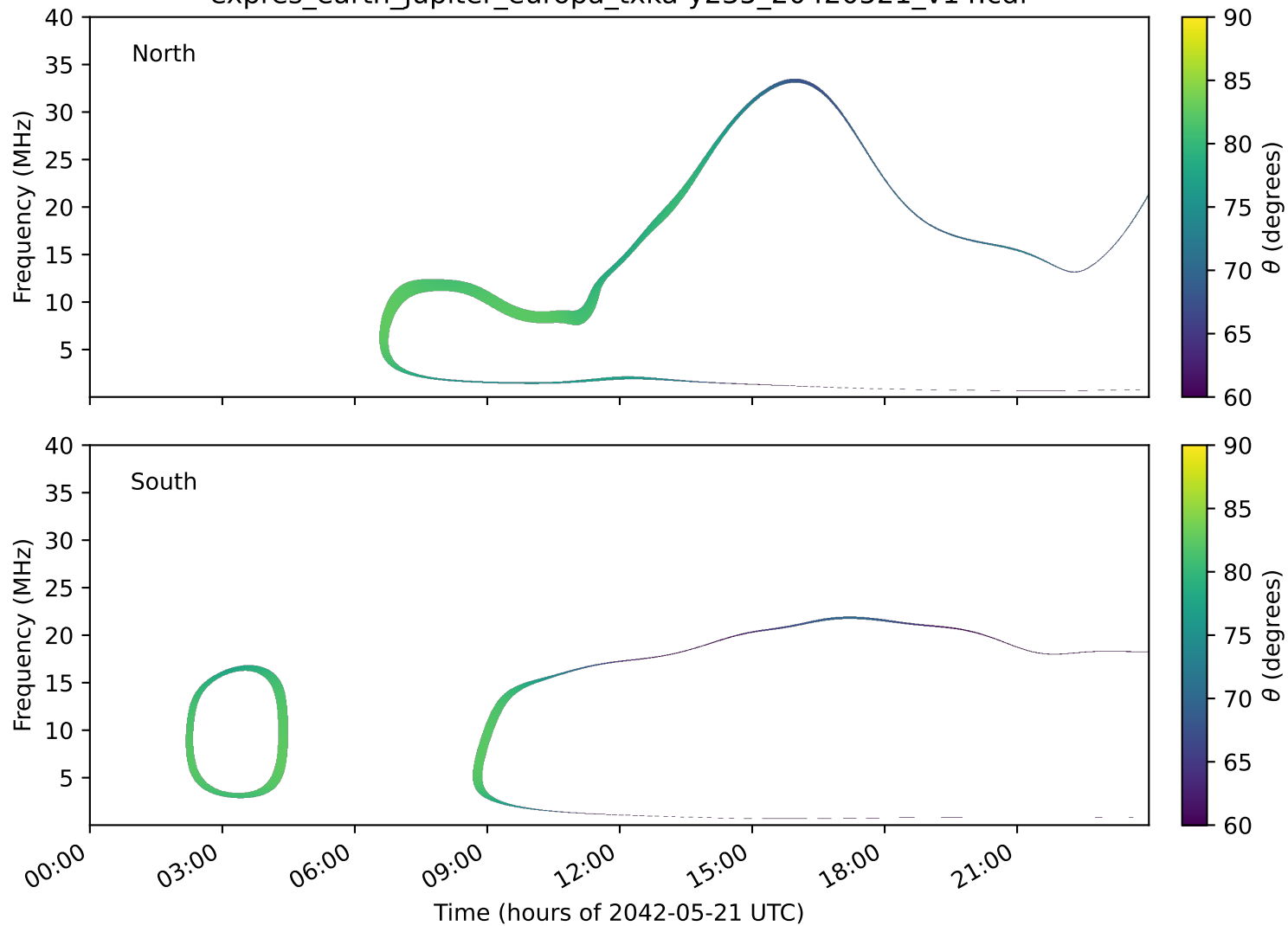
expres_earth_jupiter_europa_txka-y235_20420521_v14.cdf
