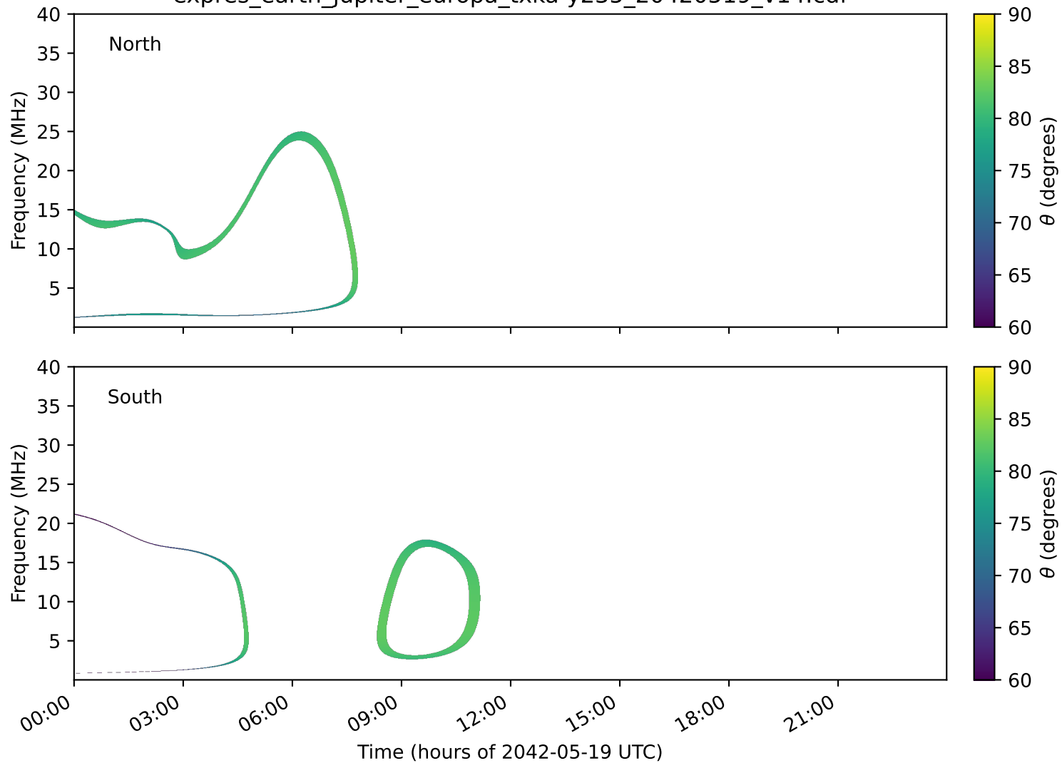
expres_earth_jupiter_europa_txka-y235_20420519_v14.cdf
