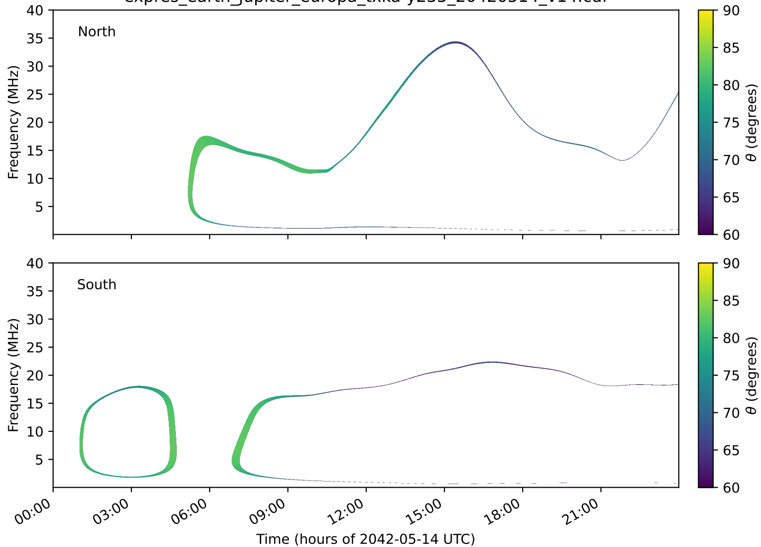
expres_earth_jupiter_europa_txka-y235_20420514_v14.cdf
