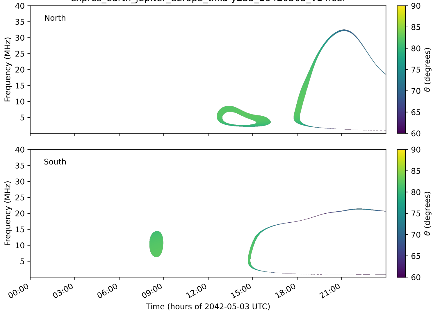
expres_earth_jupiter_europa_txka-y235_20420503_v14.cdf
