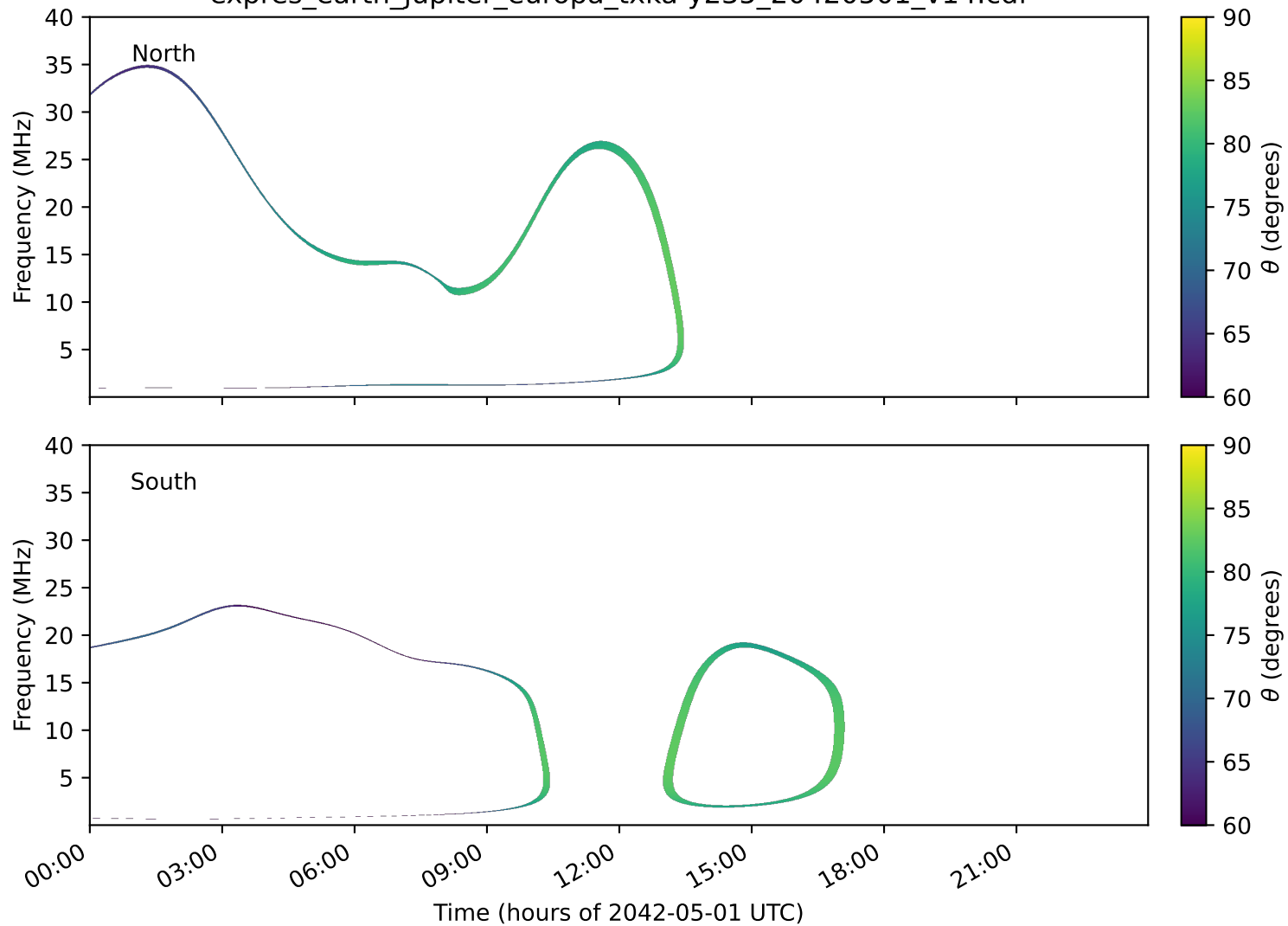
expres_earth_jupiter_europa_txka-y235_20420501_v14.cdf
