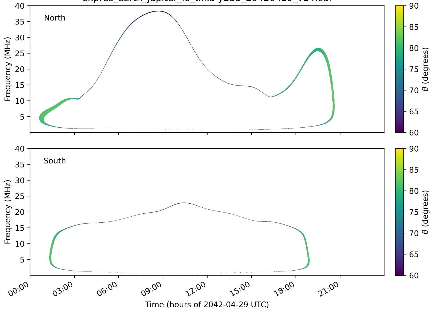
expres_earth_jupiter_io_txka-y235_20420429_v14.cdf
