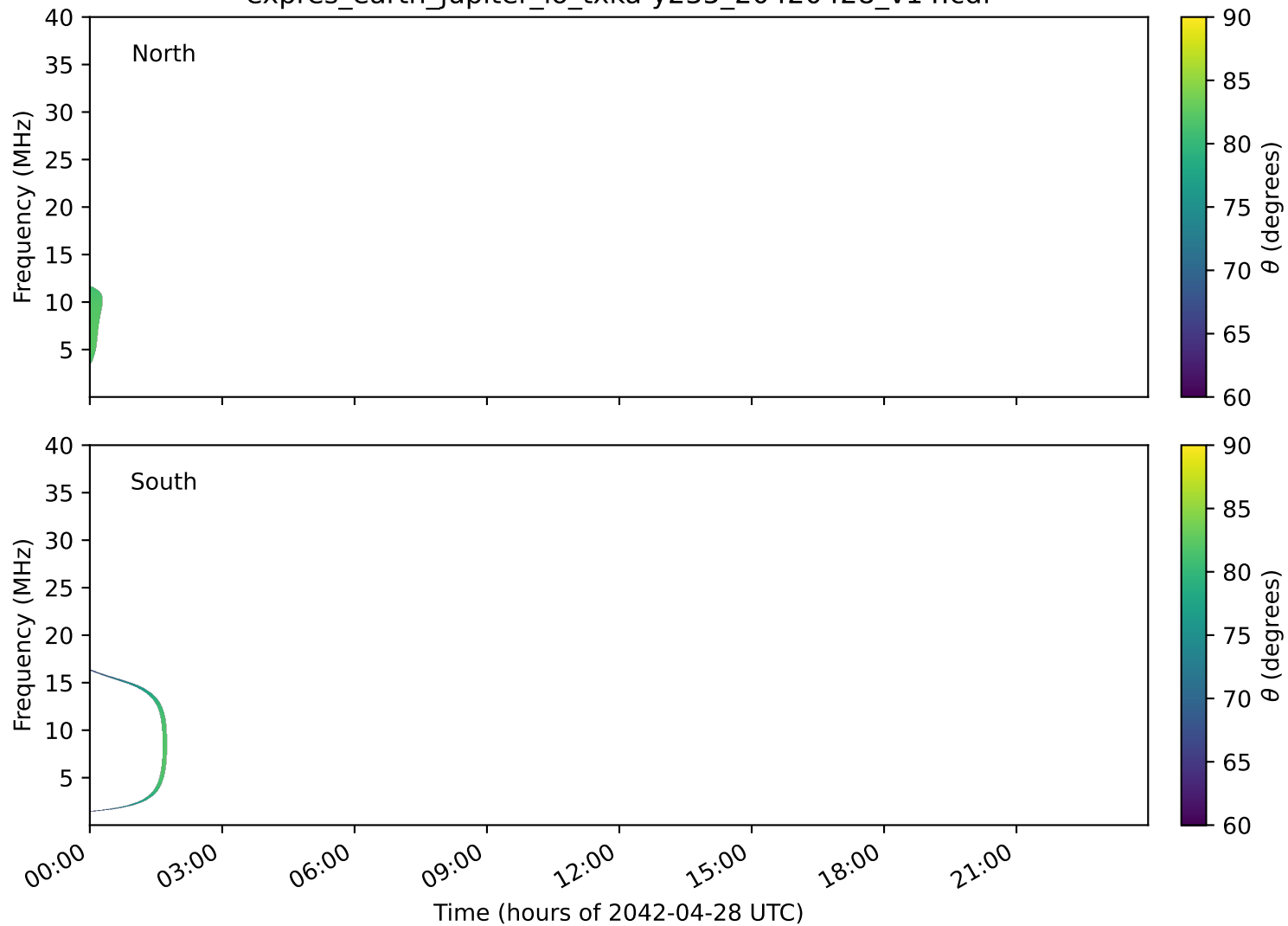
expres_earth_jupiter_io_txka-y235_20420428_v14.cdf
