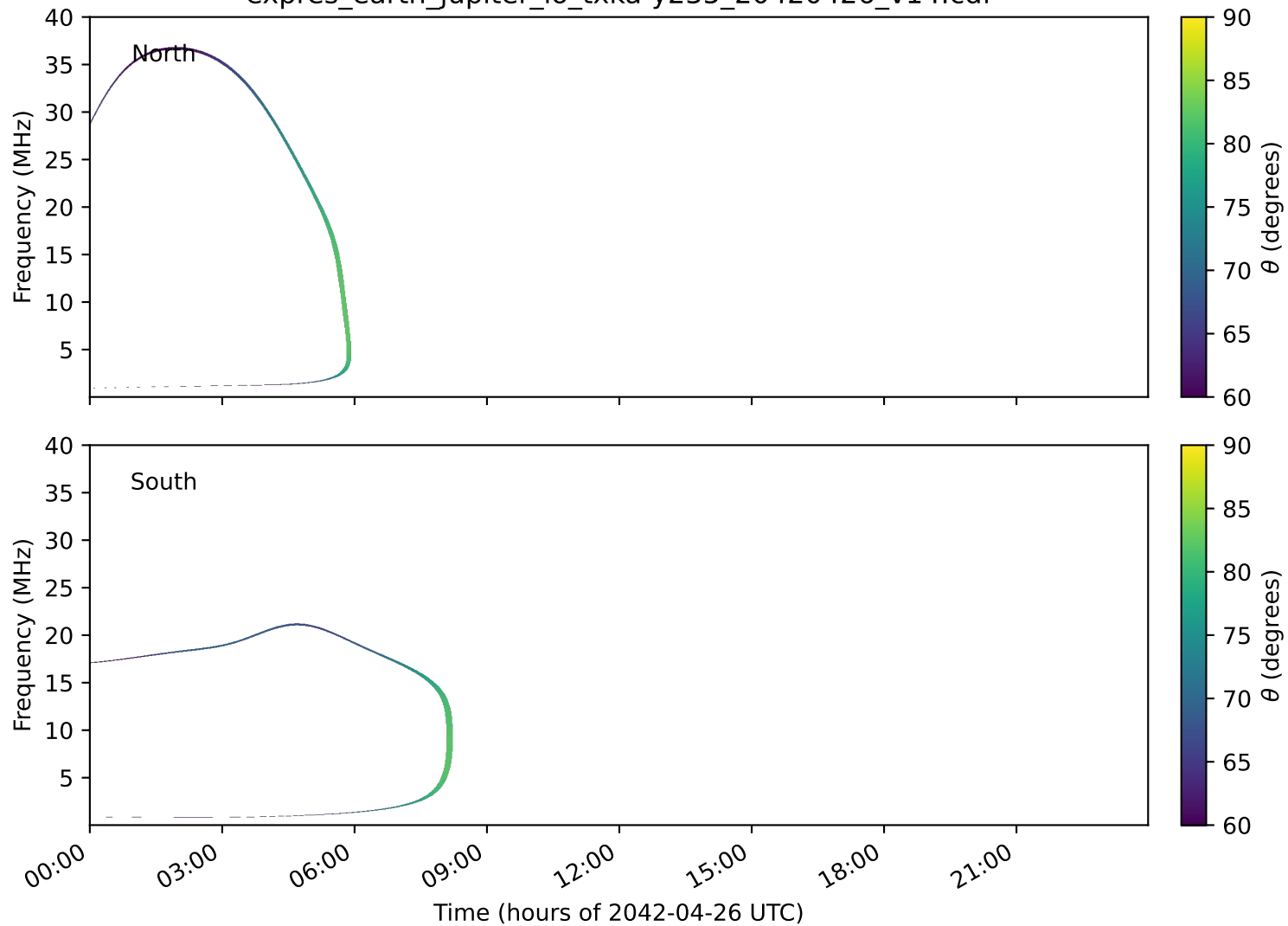
expres_earth_jupiter_io_txka-y235_20420426_v14.cdf
