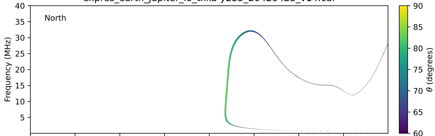
expres_earth_jupiter_io_txka-y235_20420425_v14.cdf
