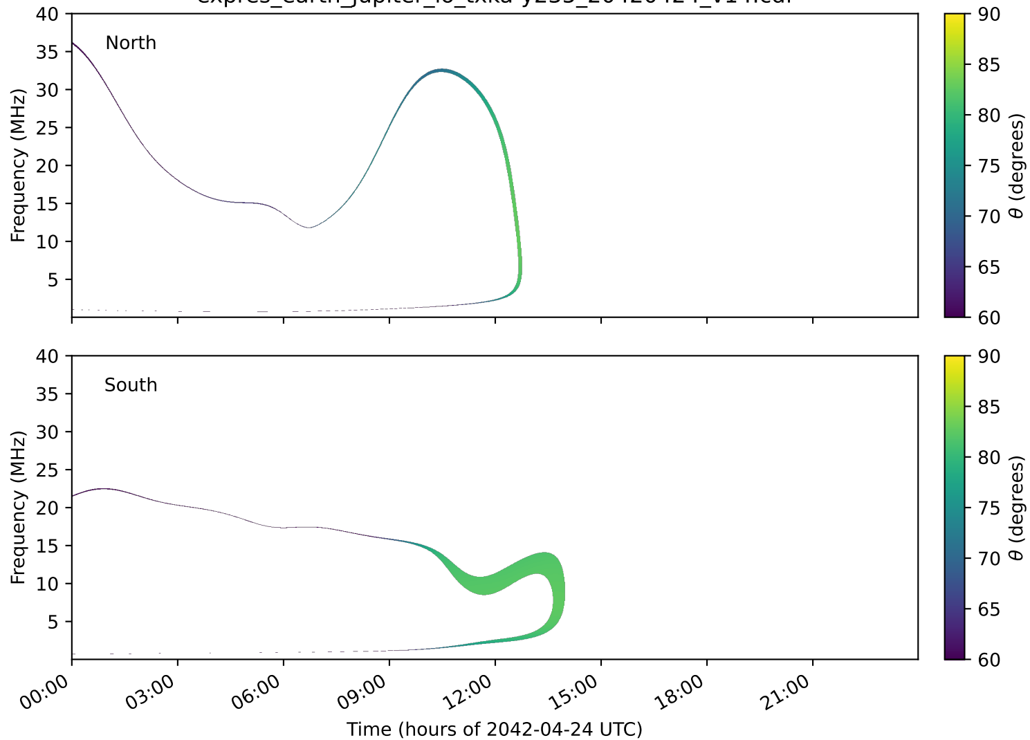
expres_earth_jupiter_io_txka-y235_20420424_v14.cdf
