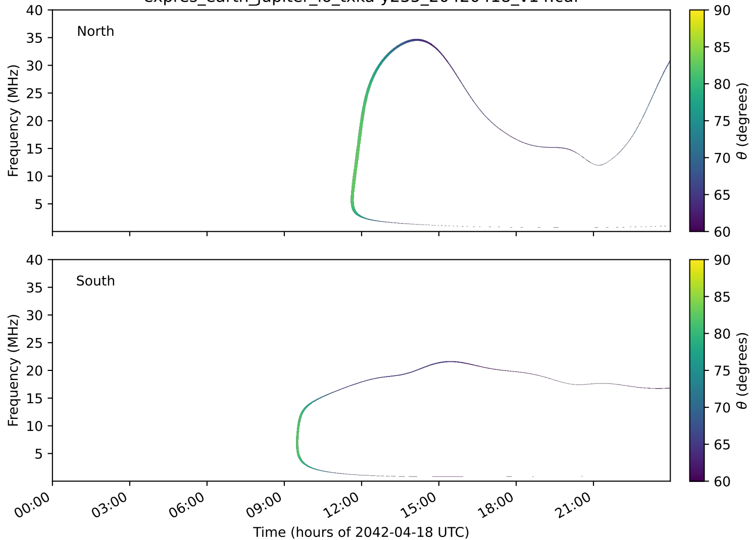
expres_earth_jupiter_io_txka-y235_20420418_v14.cdf
