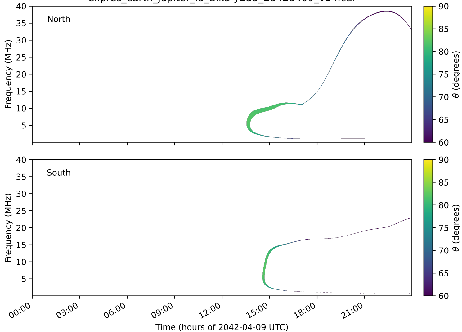
expres_earth_jupiter_io_txka-y235_20420409_v14.cdf
