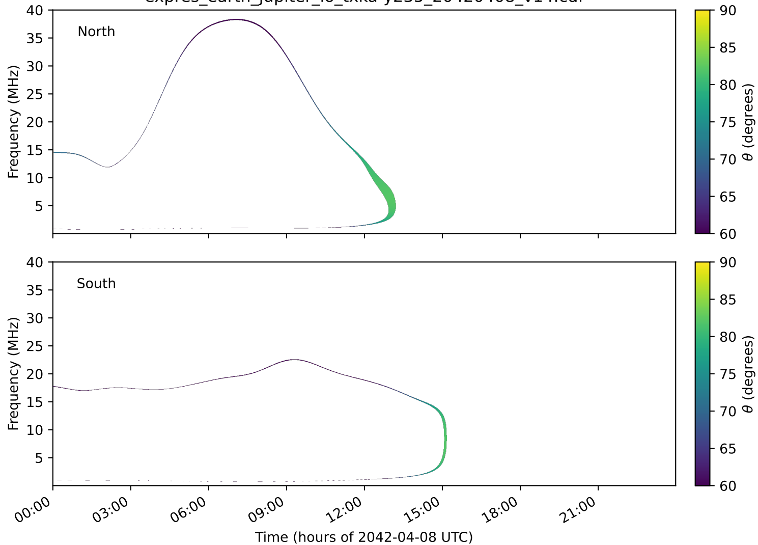
expres_earth_jupiter_io_txka-y235_20420408_v14.cdf
