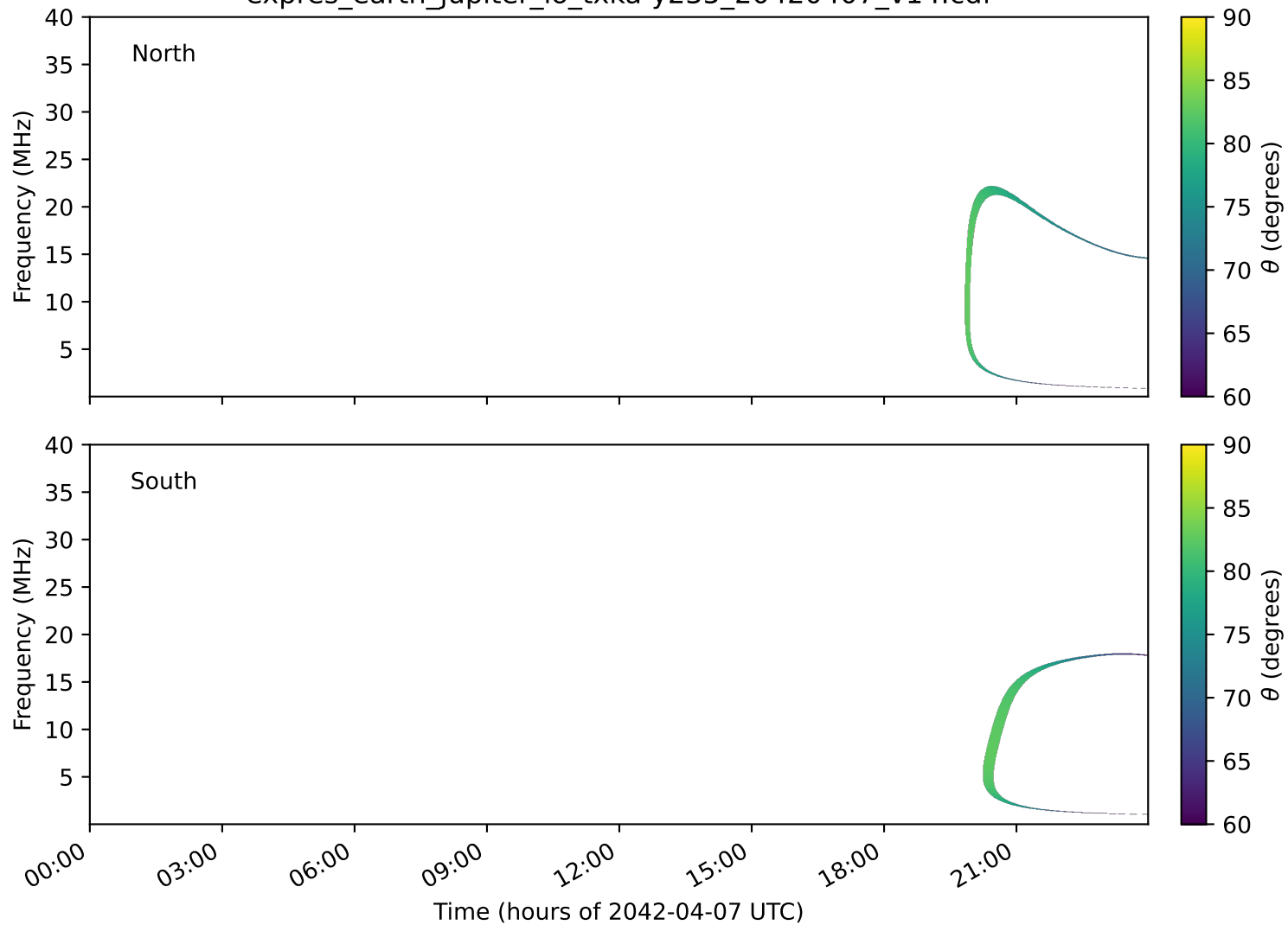
expres_earth_jupiter_io_txka-y235_20420407_v14.cdf
