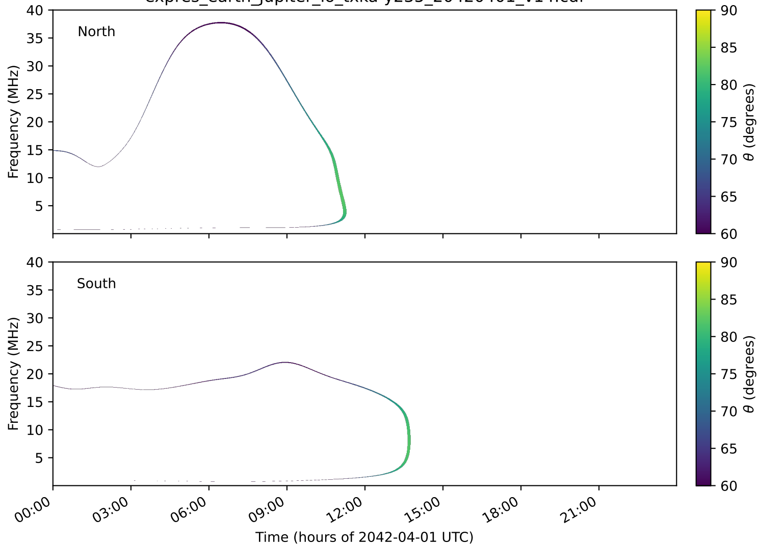
expres_earth_jupiter_io_txka-y235_20420401_v14.cdf
