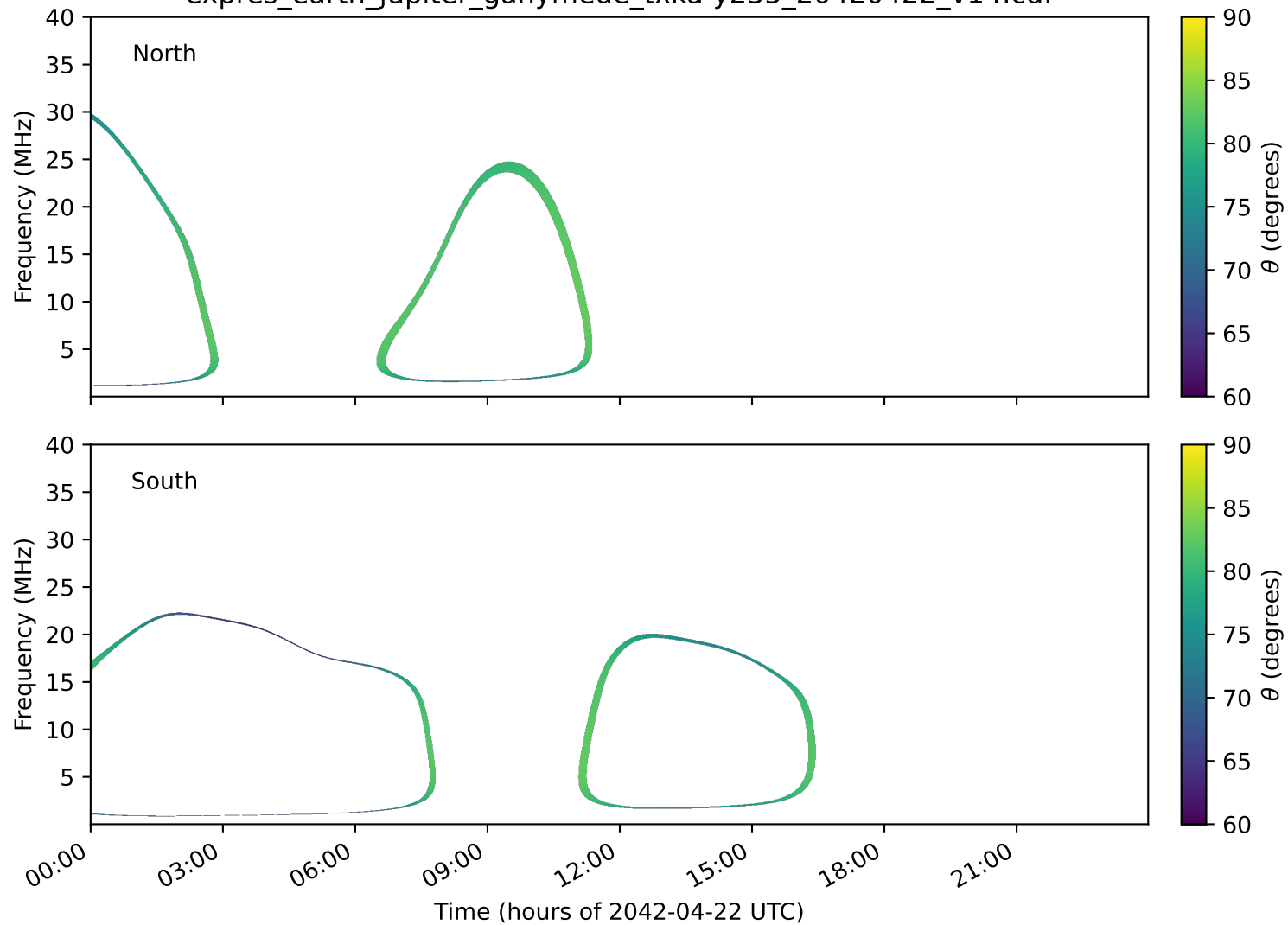
expres_earth_jupiter_ganymede_txka-y235_20420422_v14.cdf
