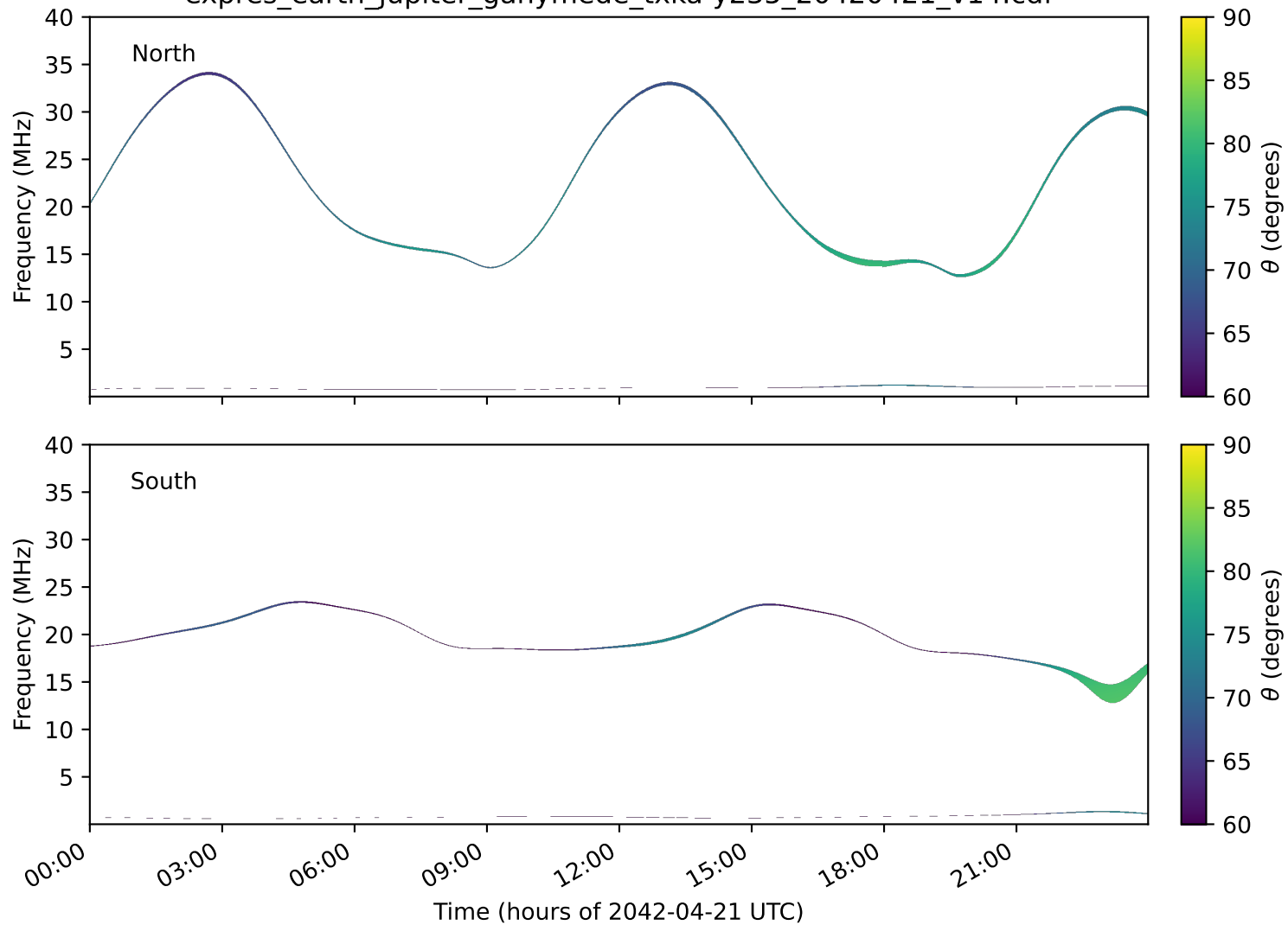
expres_earth_jupiter_ganymede_txka-y235_20420421_v14.cdf
