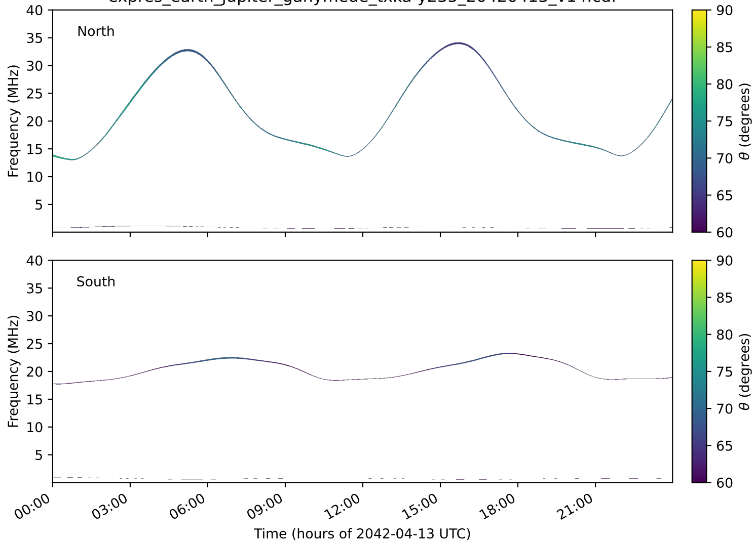
expres_earth_jupiter_ganymede_txka-y235_20420413_v14.cdf
