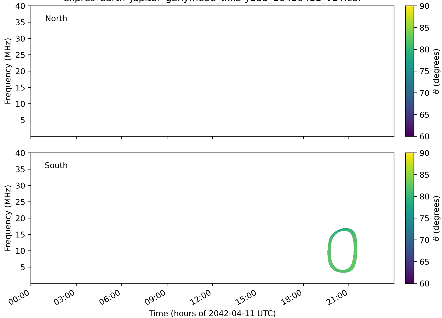
expres_earth_jupiter_ganymede_txka-y235_20420411_v14.cdf
