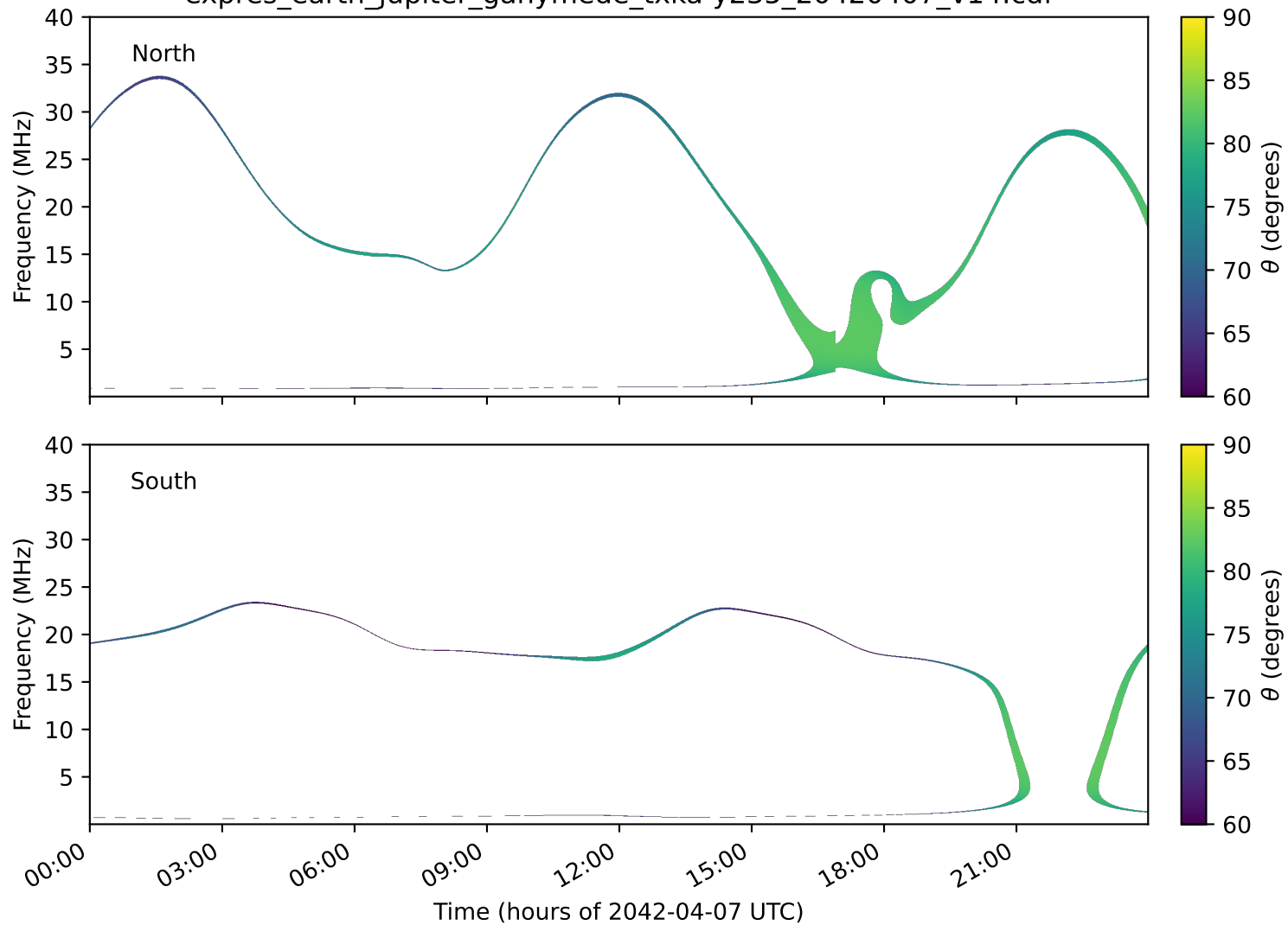
expres_earth_jupiter_ganymede_txka-y235_20420407_v14.cdf
