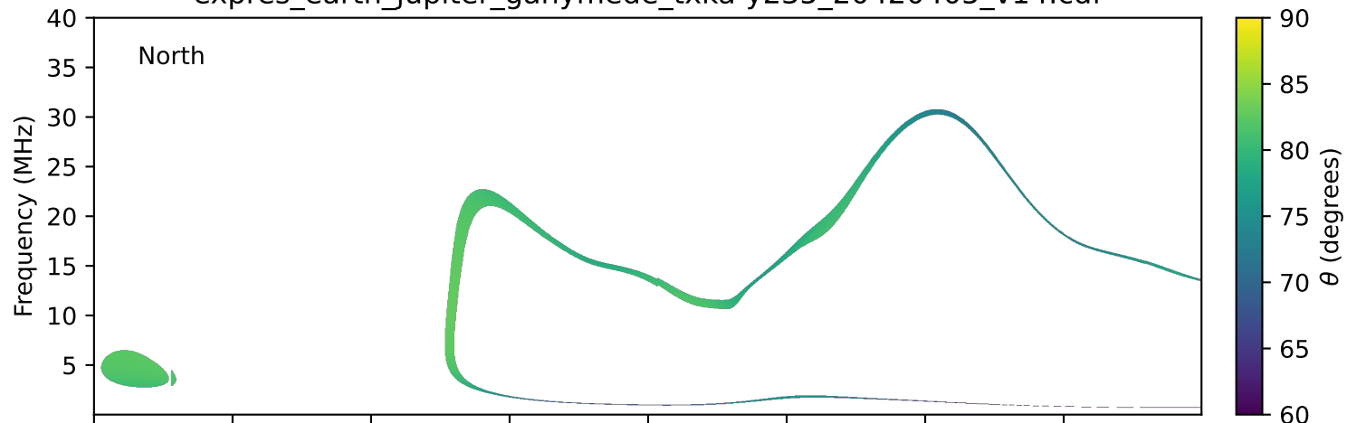
expres_earth_jupiter_ganymede_txka-y235_20420405_v14.cdf
