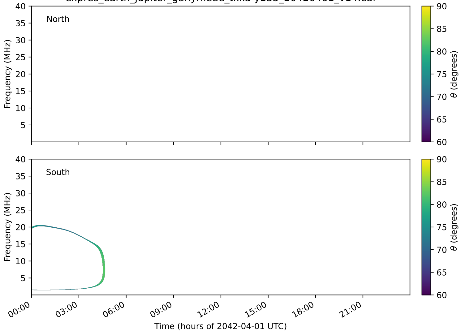
expres_earth_jupiter_ganymede_txka-y235_20420401_v14.cdf
