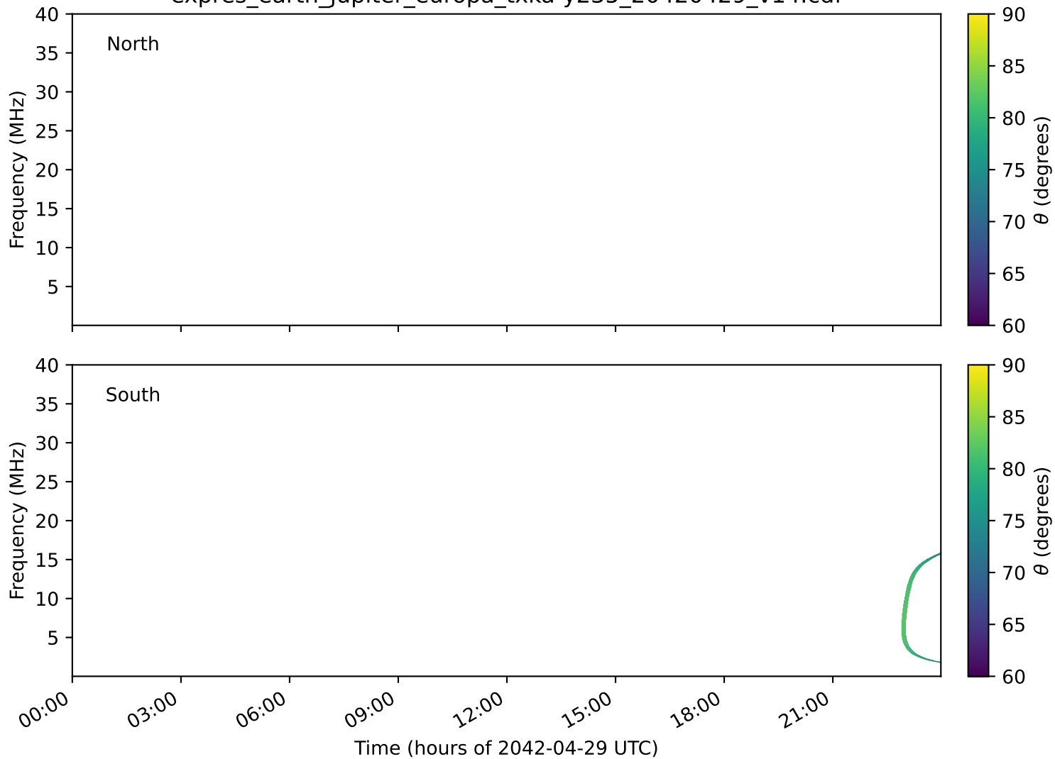
expres_earth_jupiter_europa_txka-y235_20420429_v14.cdf
