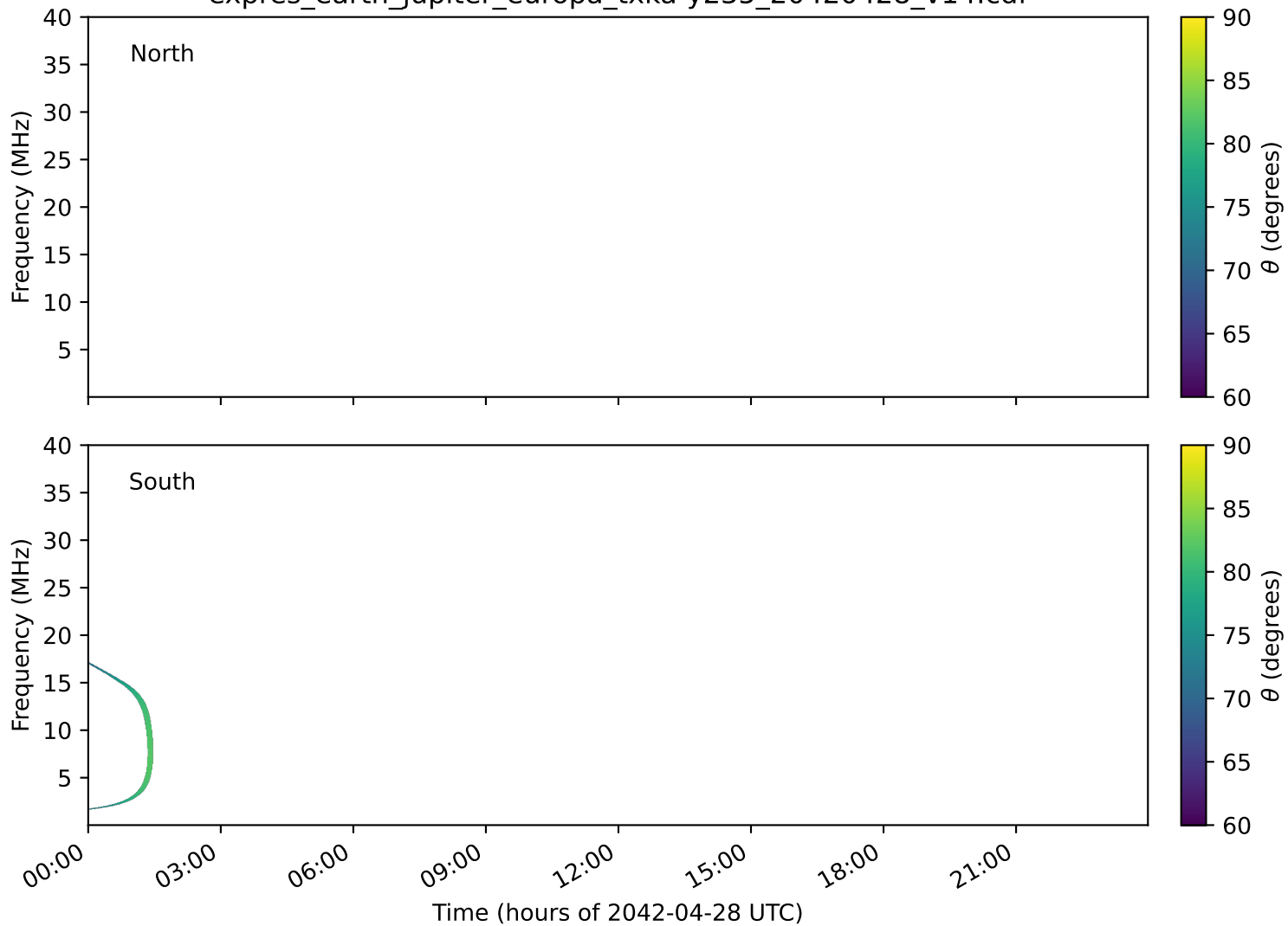
expres_earth_jupiter_europa_txka-y235_20420428_v14.cdf
