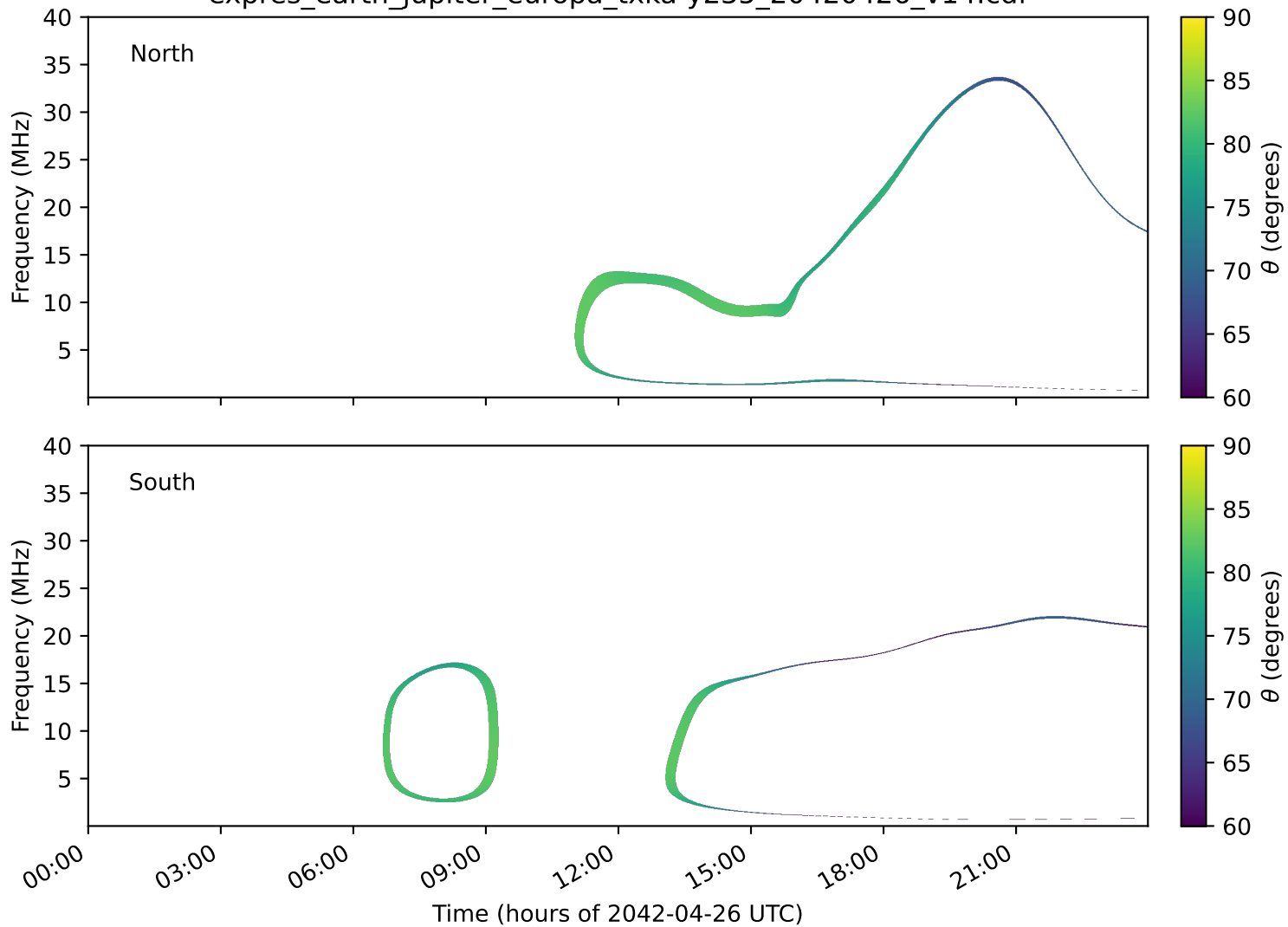
expres_earth_jupiter_europa_txka-y235_20420426_v14.cdf
