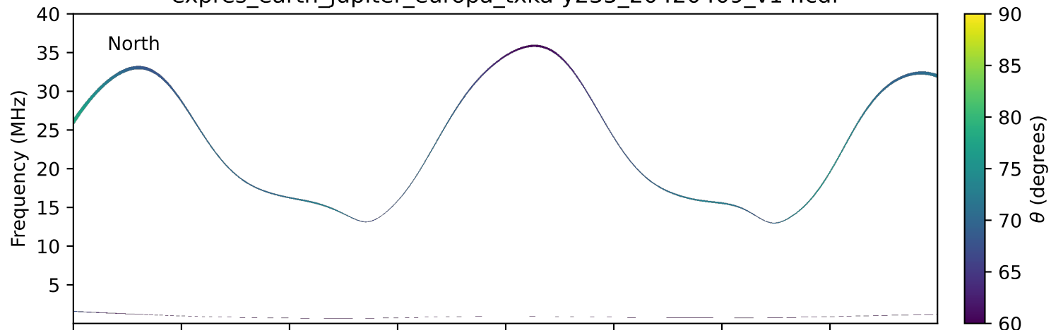
expres_earth_jupiter_europa_txka-y235_20420409_v14.cdf
