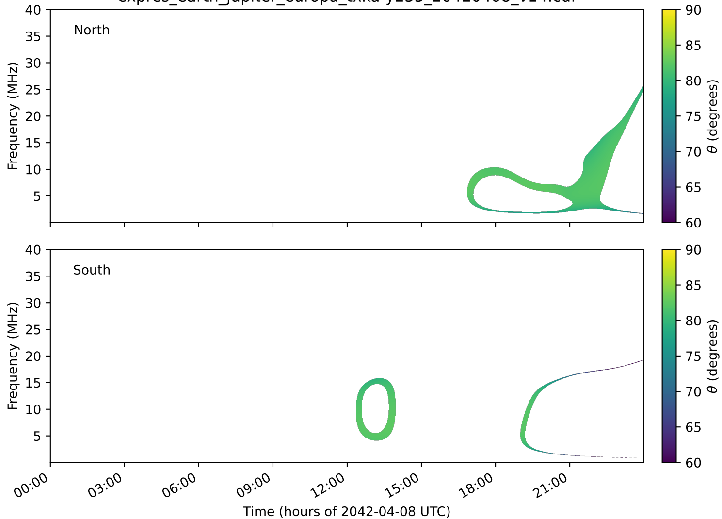
expres_earth_jupiter_europa_txka-y235_20420408_v14.cdf
