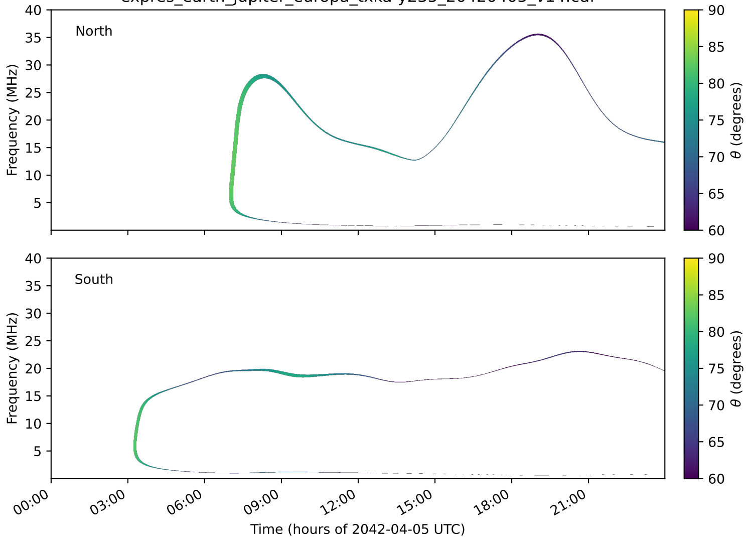
expres_earth_jupiter_europa_txka-y235_20420405_v14.cdf
