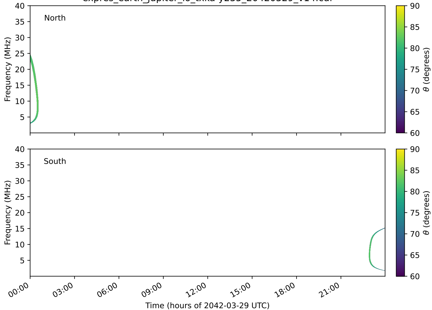
expres_earth_jupiter_io_txka-y235_20420329_v14.cdf
