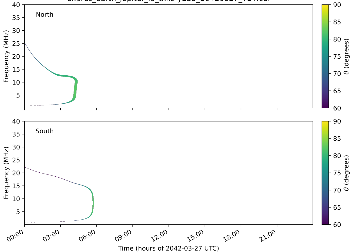
expres_earth_jupiter_io_txka-y235_20420327_v14.cdf
