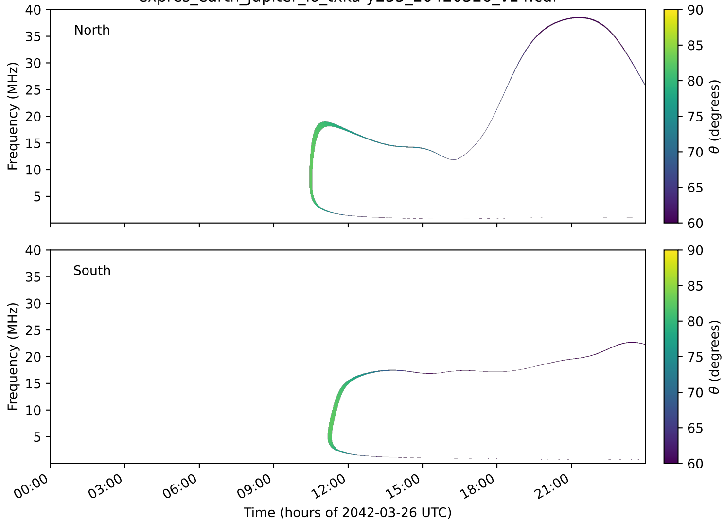
expres_earth_jupiter_io_txka-y235_20420326_v14.cdf
