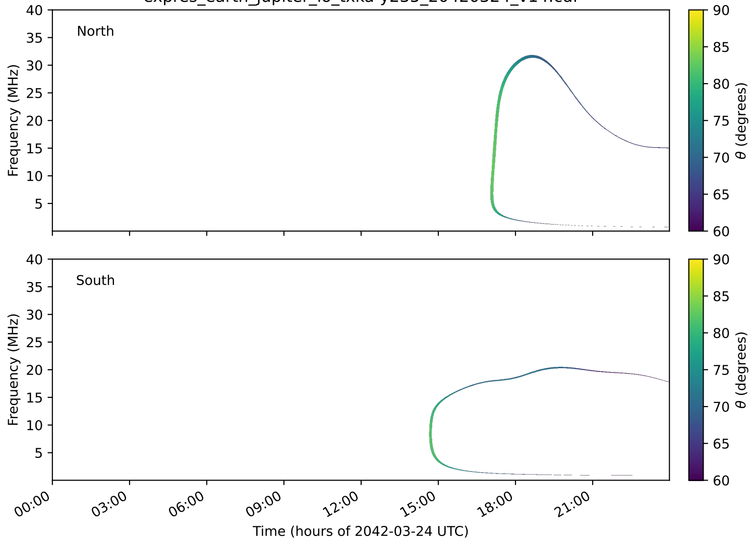
expres_earth_jupiter_io_txka-y235_20420324_v14.cdf
